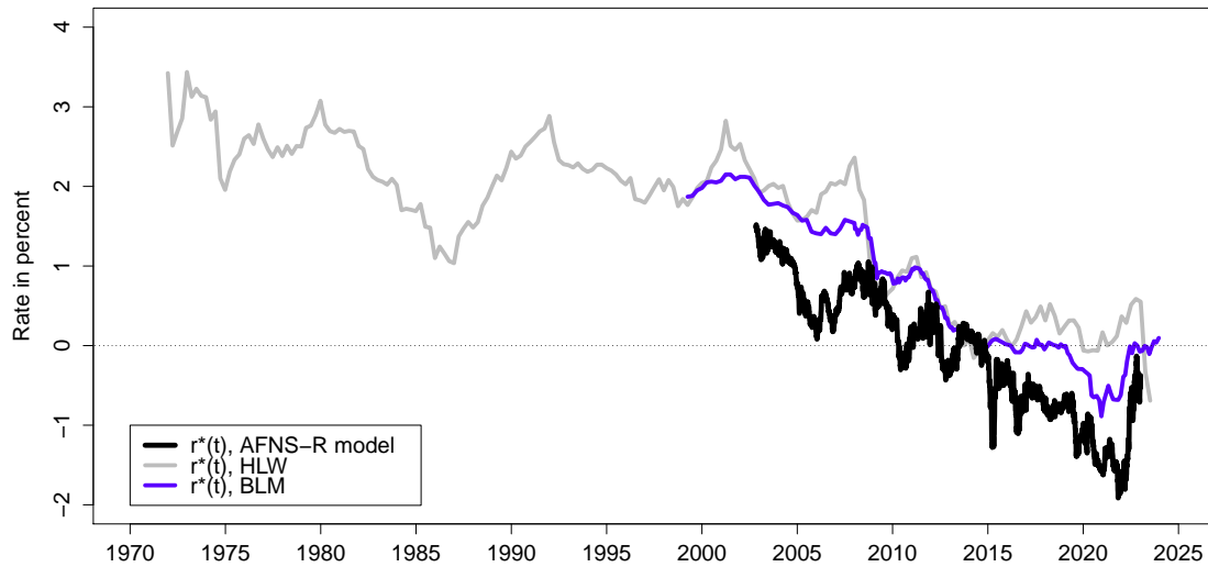
Figure 14: Comparison with Macro-Based Estimates of r^*
