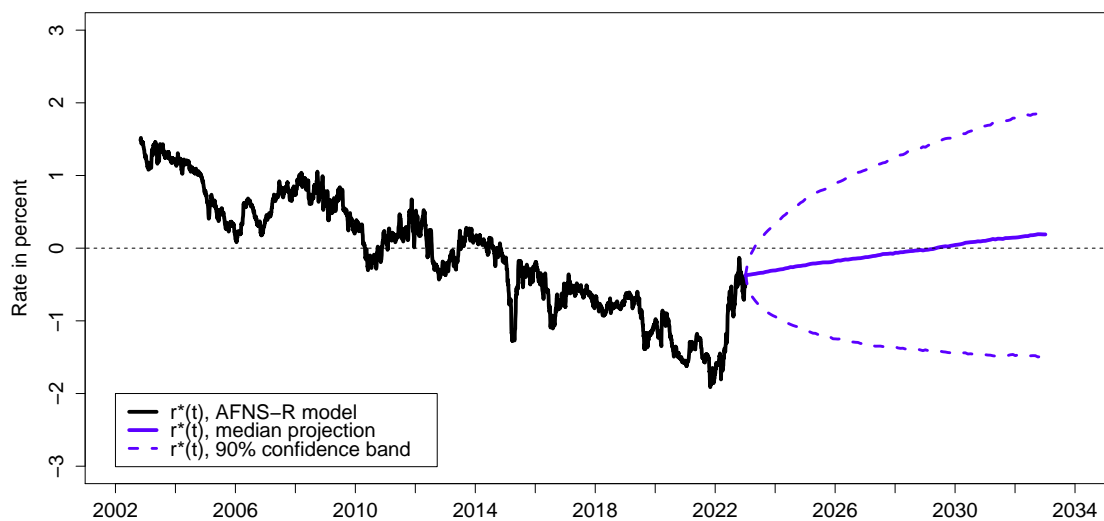
Figure 15: Ten-Year Projections of r^* from AFNS-R Model
